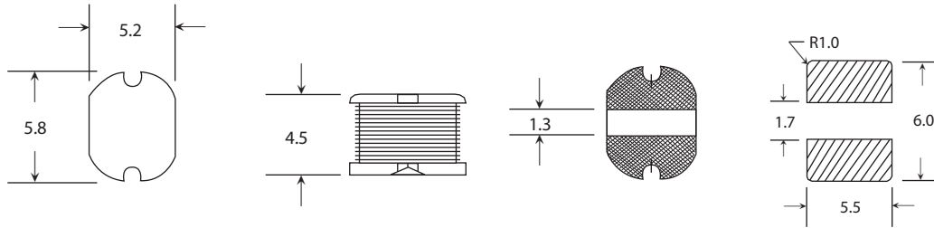
Pad Layout
